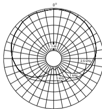
Polar Pattern (d:fine™ 4088 & 4088 Omni Headset types)
